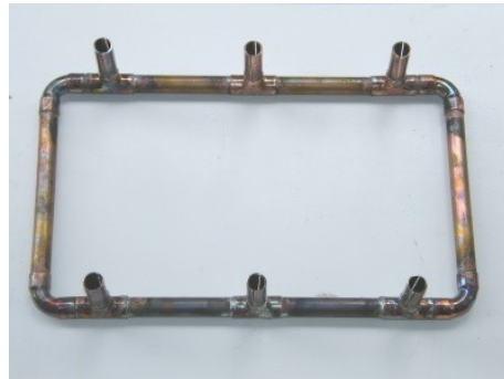
Fig. 6: Copper tube structure
