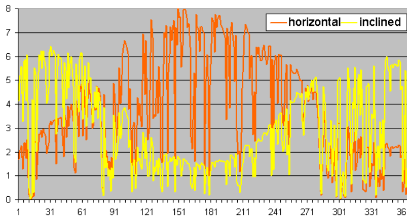
Fig. 3: Daily solar radiation in Nigran during year 2005 (Kwh/m²)
